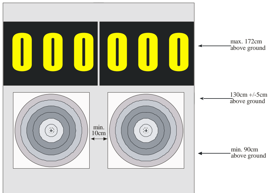
2 x 80cm 6-ring faces with the scoringzones 5-10
